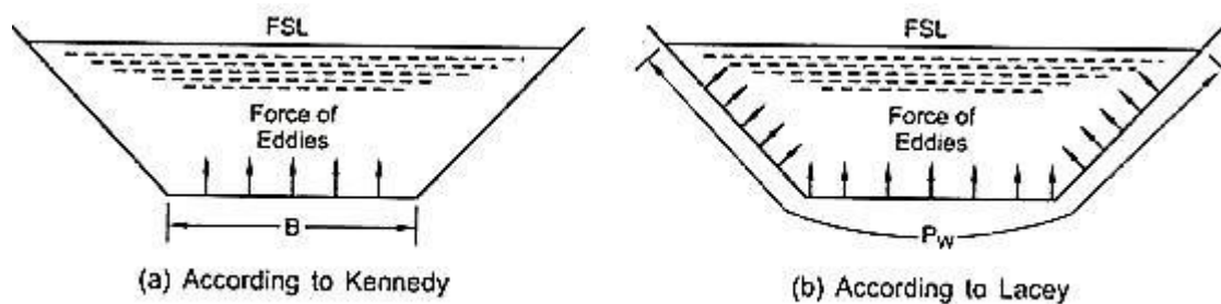
Fig. 9.2. Lacey's theory
