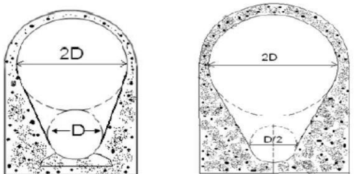
New/ Modified Egg shaped Sewer
