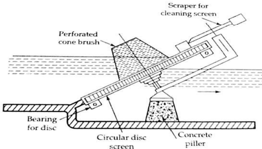
Fig. 9.3. Reinsch-Wurl screen (disc type fine screen).
