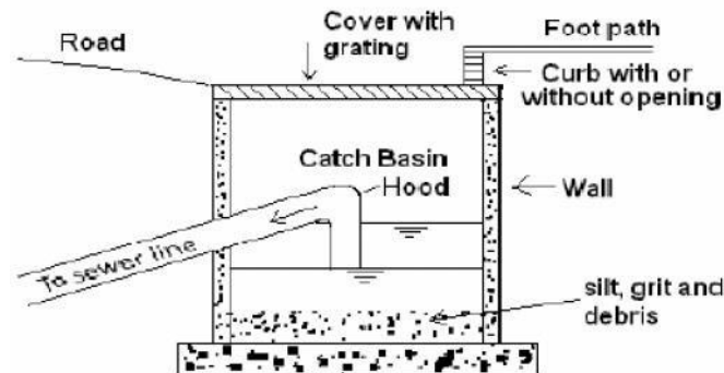
Catch Basins
